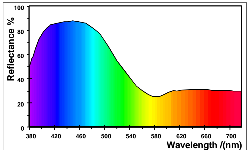
Figure 28: Reflectance spectrum for a blue surface
